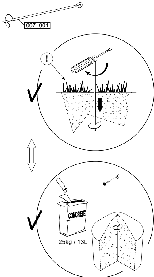
Twist-Anchor
